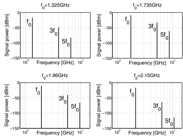
Fig. 10. Spectrum of the differential output signal.
