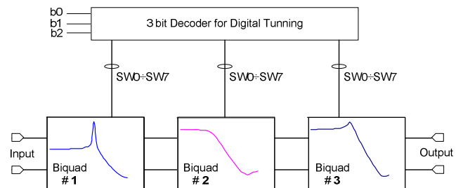
Fig. 1. 6 th order LPF structure
