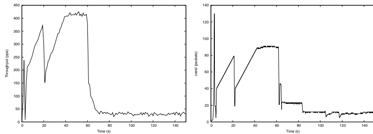
Fig. 8. Vegas with an additional 200ms RTT in an initially uncontended WLAN with additional fws introduced around 60s: (a) Throughput. (b) Cwnd.
