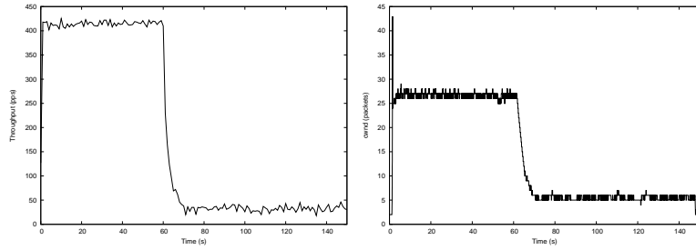
Fig. 7. Vegas with 5ms additional RTT in an initially uncontended WLAN with additional fws introduced around 60s: (a) throughput, (b) cwnd.
